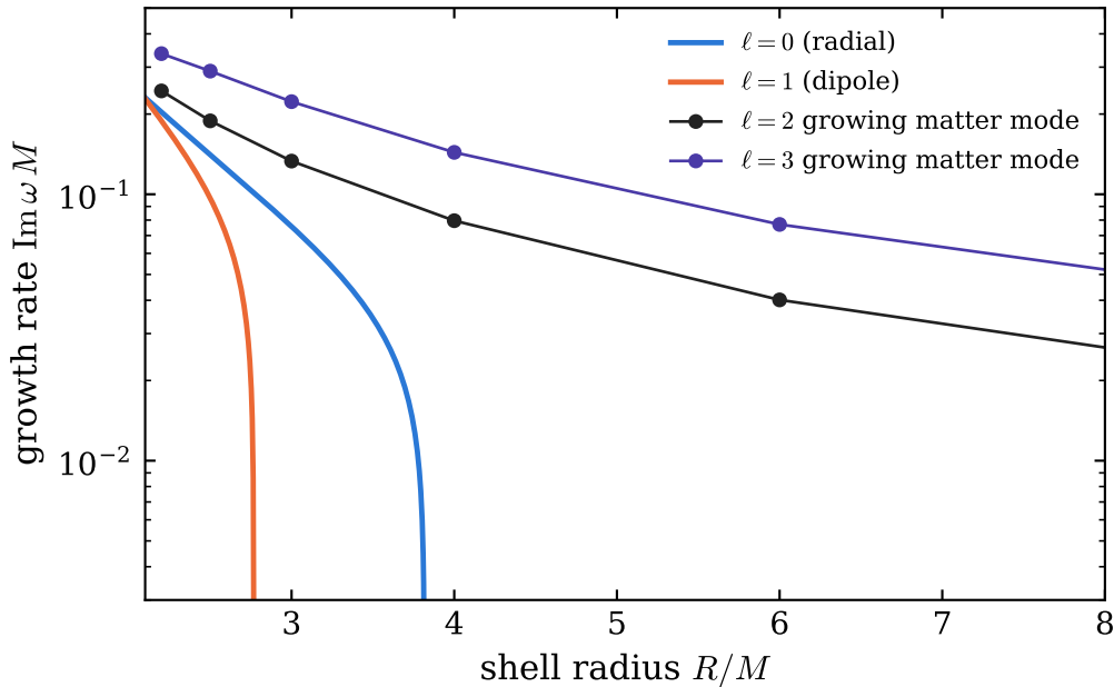
Instability rates of the static shell, \Gamma = 2
